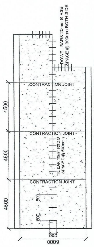
CONSTRUCTION/LONGITUDINAL JOINT ON CARRIAGE WAY
