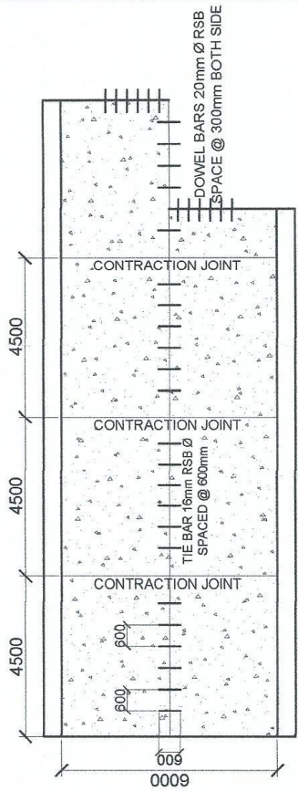
TYPICAL ROADWAY DETAIL
