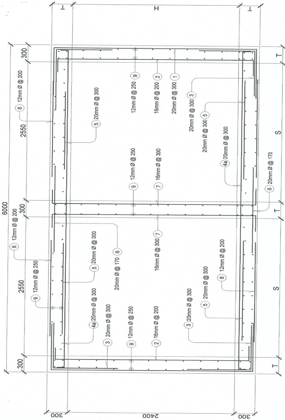
SECTION-DOUBLE BARREL
